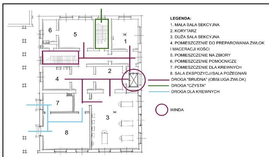
Fig. 5. Concept for the expansion of the prosectorium at the August Bier Hospital, functional diagram of the ground floor. Authors' own illustration based on archival materials 165 .
